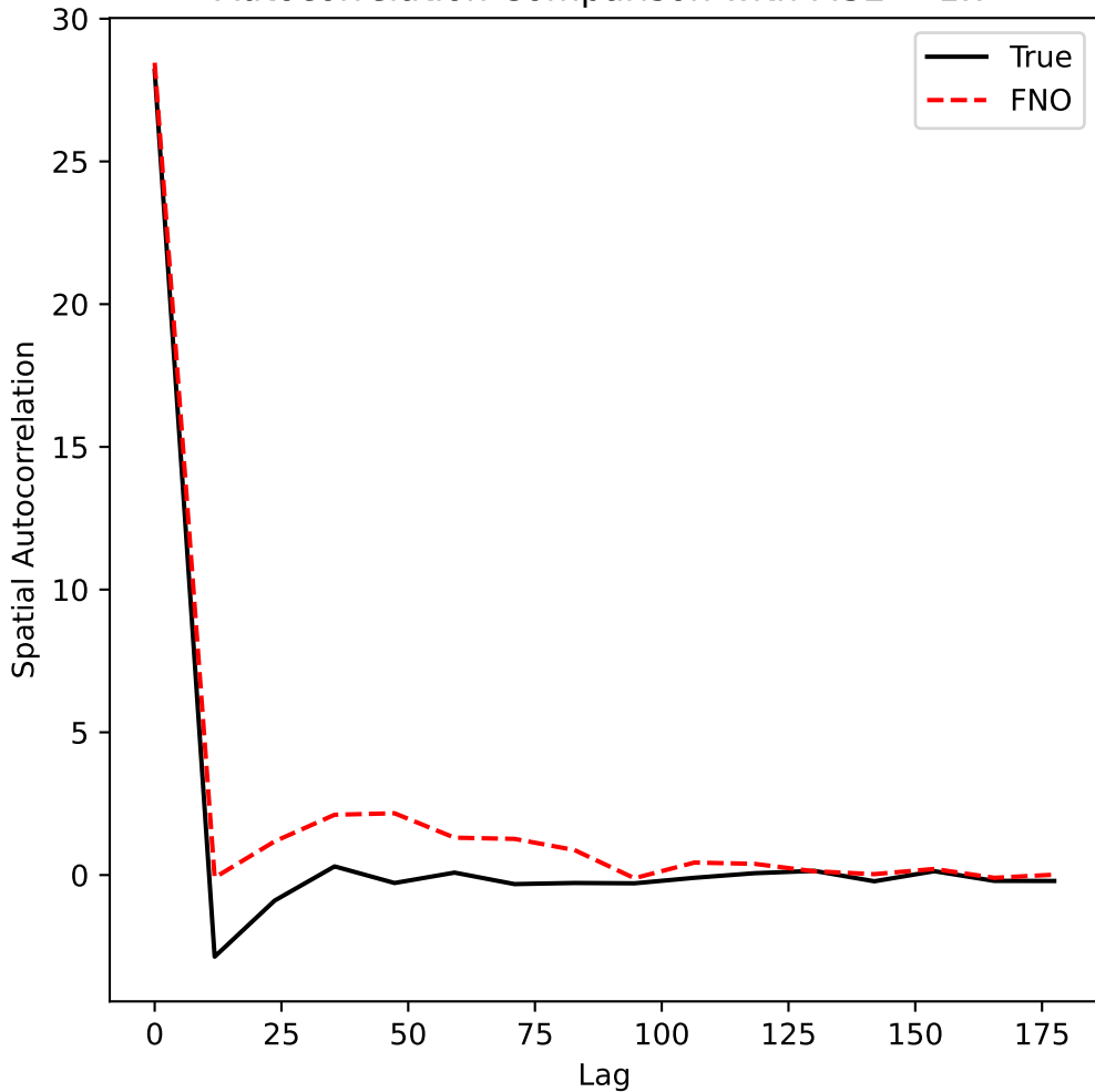
Autocorrelation Comparison with MSE = 1.7
