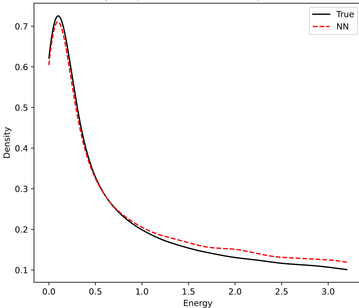
TKE Density Comparison with KS: 0.027, p-value: 5.4e-122
