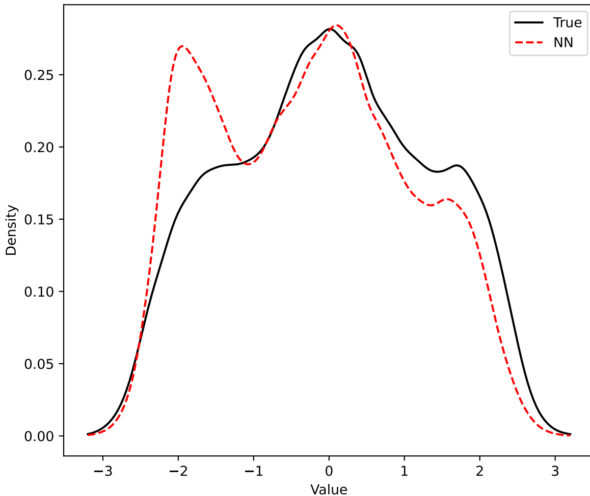
Empirical Density Comparison with KS: 0.076, p-value: 0
