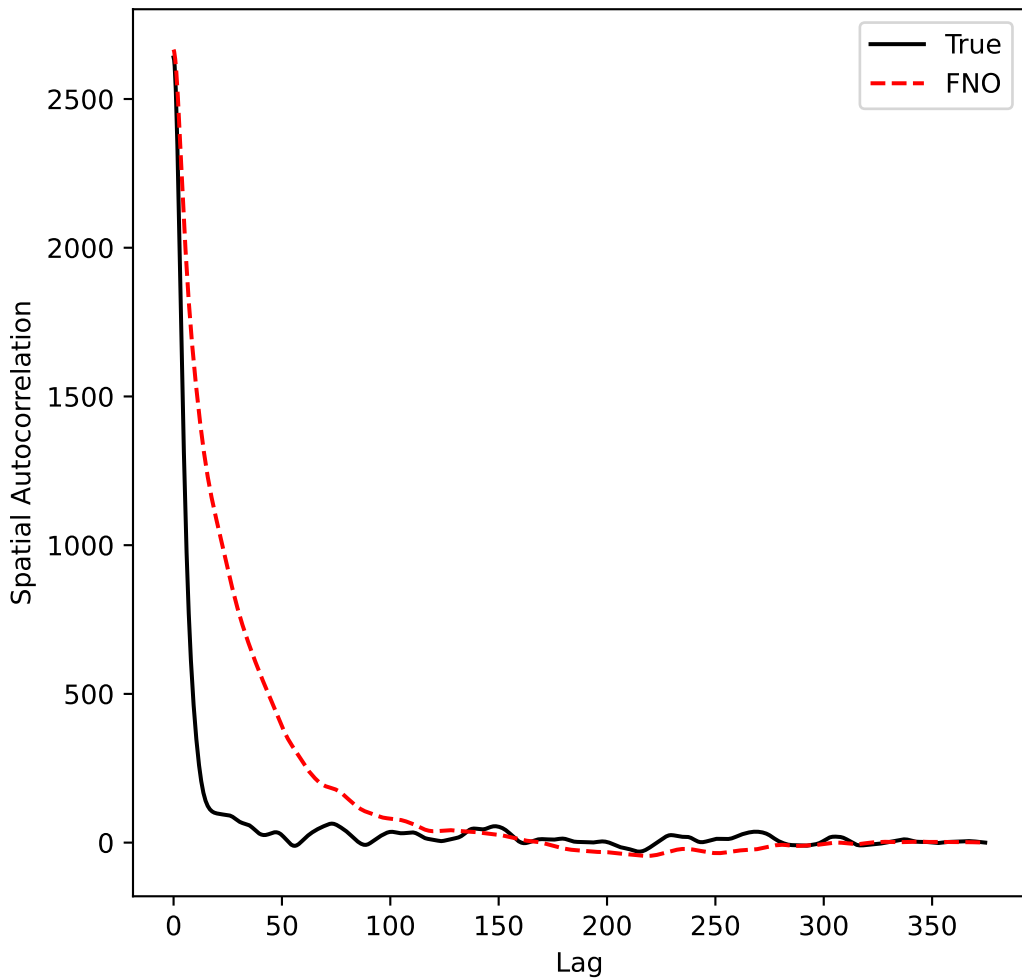
Autocorrelation Comparison with MSE = 9\text{e}+04
